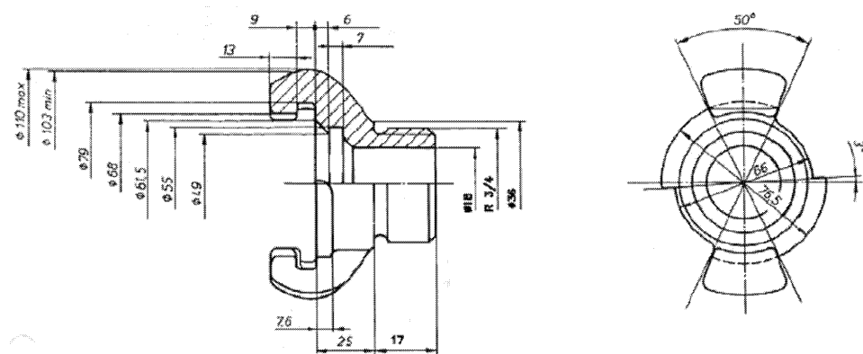
Figure A III1 The water filling adapters
